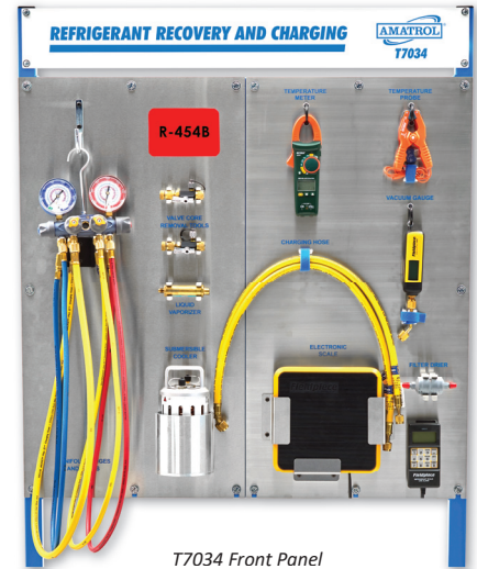
T7034 Front Panel
